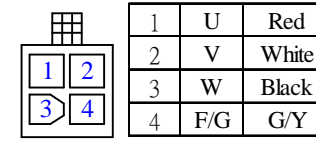
Motor Connection
